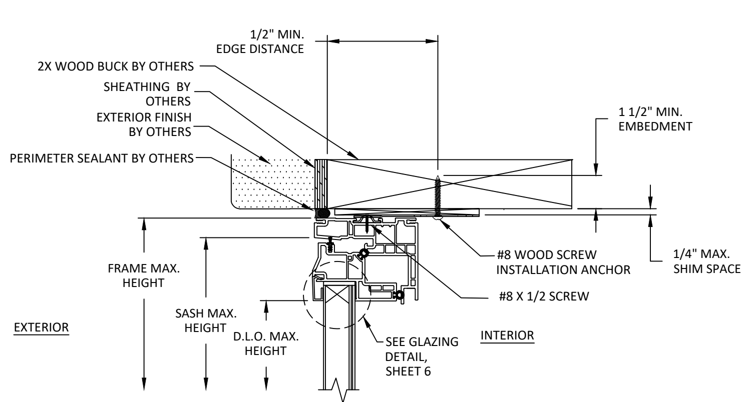
A 5 VERTICAL SECTION CLIP INSTALLATION WOOD SUBSTRATE
