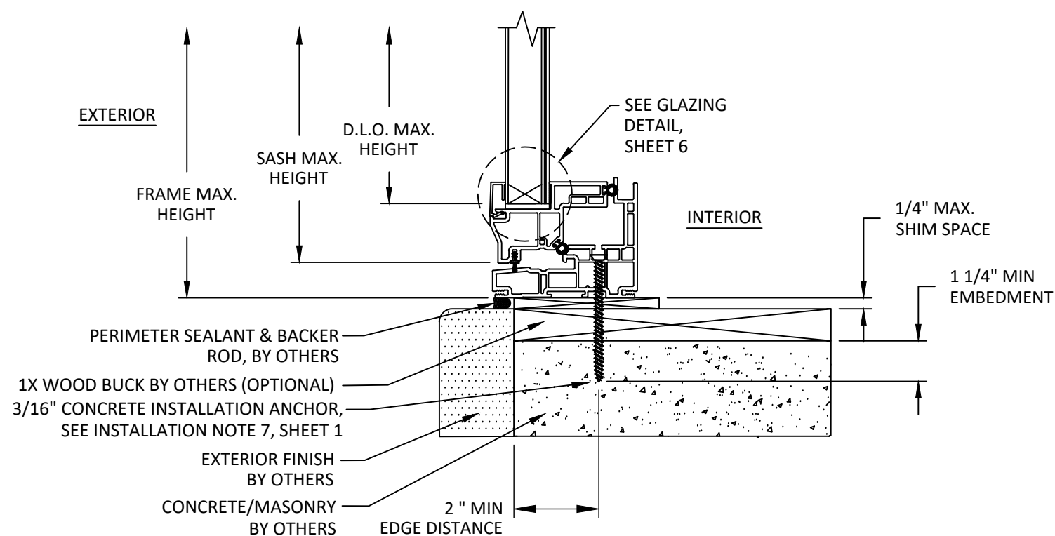
C 4 VERTICAL SECTION THROUGH FRAME INSTALLATION CMU/CONCRETE SUBSTRATE
